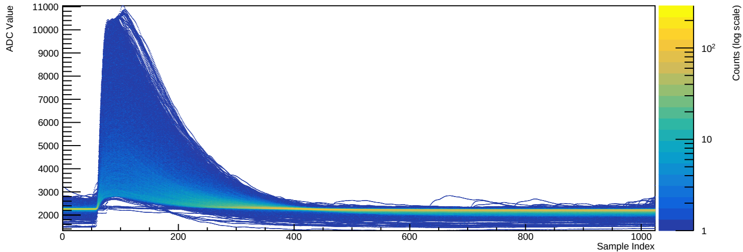
Run 039500 - Channel 2081 (n=8788 waveforms)
