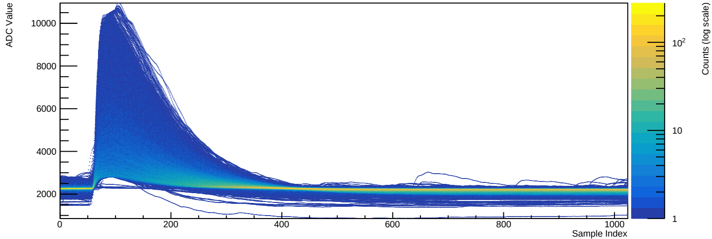
Run 039501 - Channel 2081 (n=9041 waveforms)
