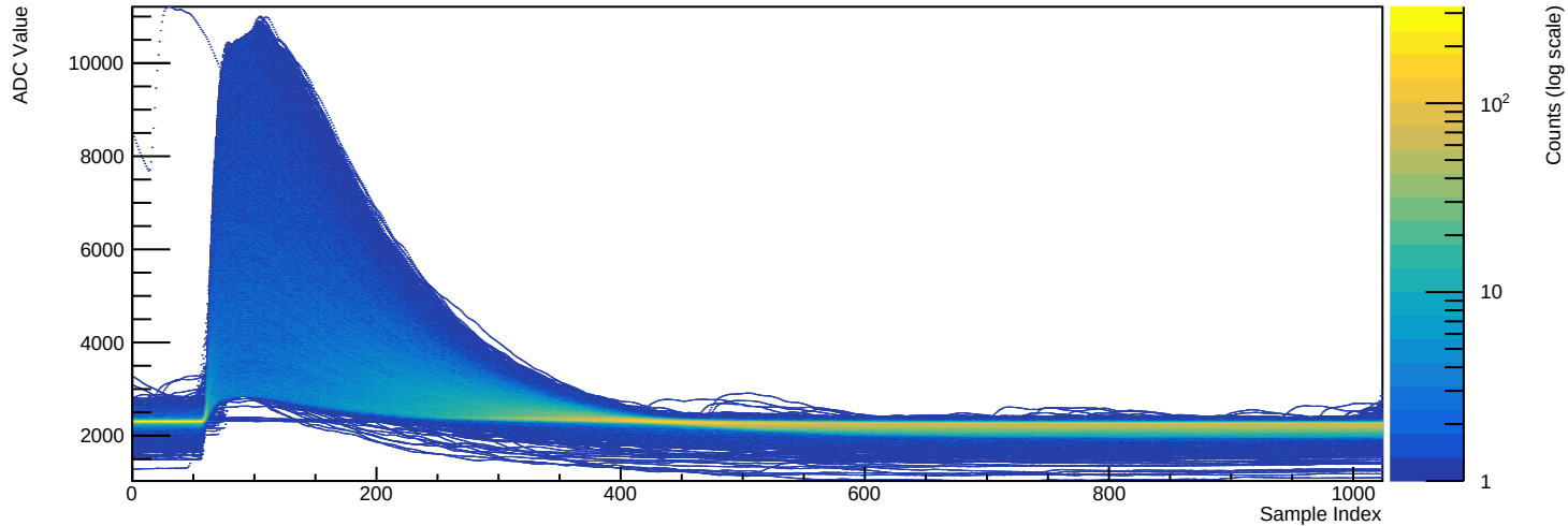
Run 039512 - Channel 2081 (n=12170 waveforms)
