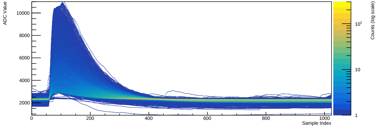
Run 039519 - Channel 2081 (n=10222 waveforms)
