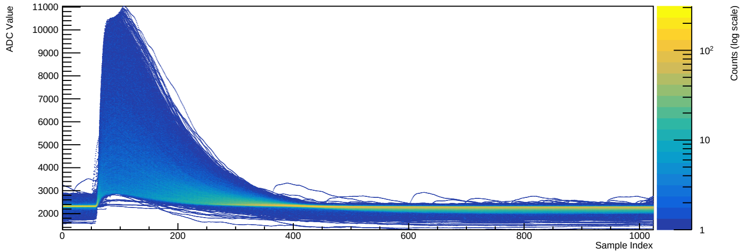
Run 039521 - Channel 2081 (n=9962 waveforms)
