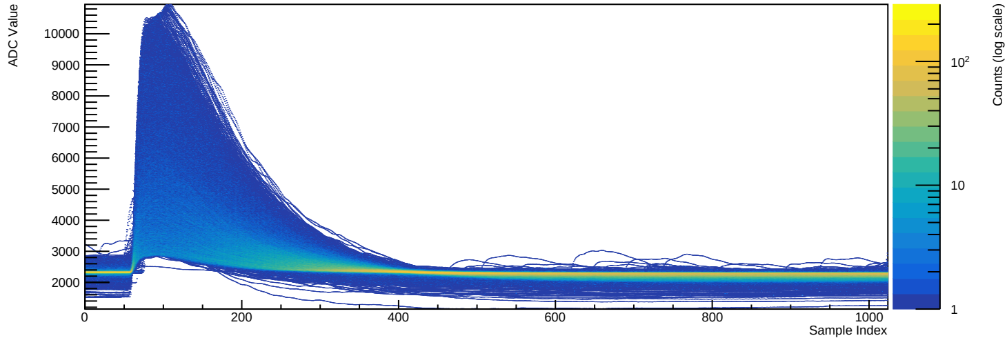
Run 039522 - Channel 2081 (n=9776 waveforms)
