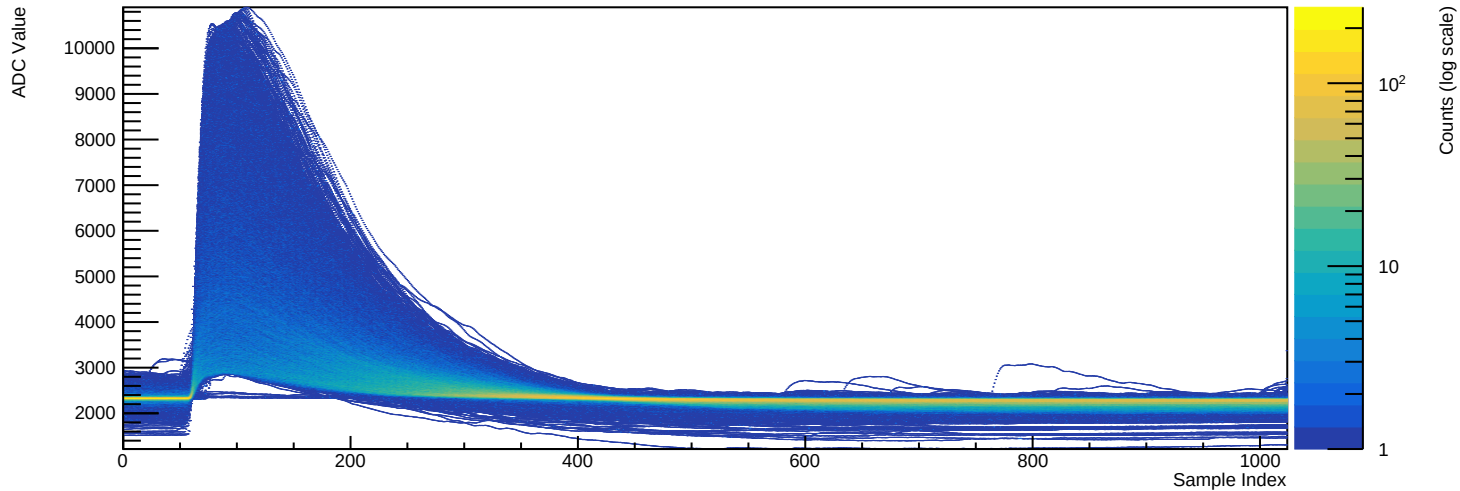
Run 039527 - Channel 2081 (n=8947 waveforms)
