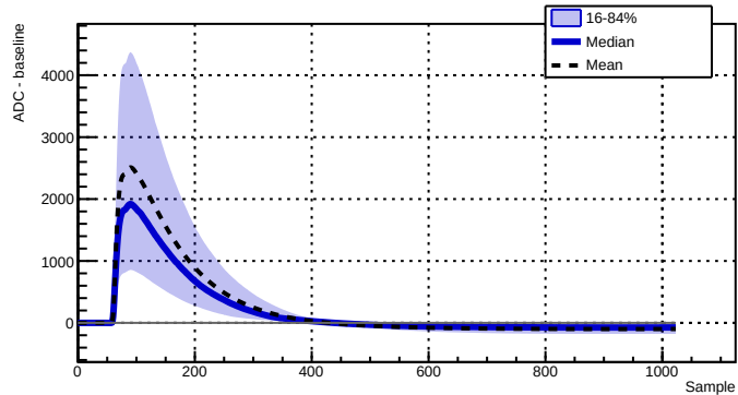
Run 039501 - Channel 2080 - 7369 waveforms
