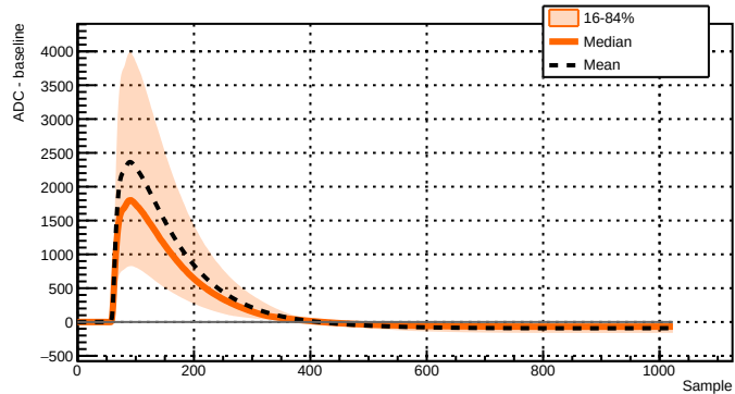
Run 039501 - Channel 2081 - 9041 waveforms
