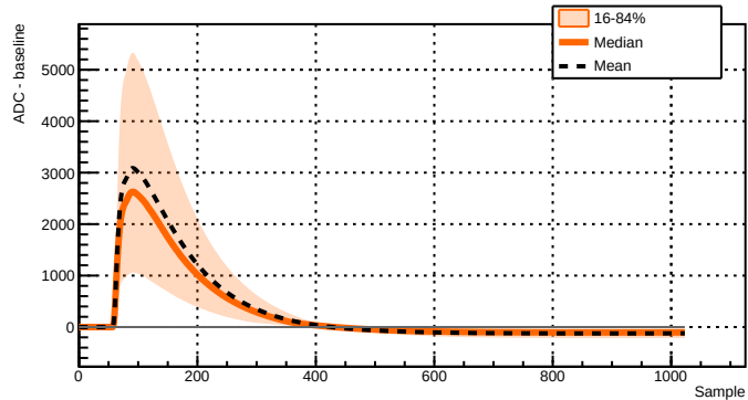
Run 039508 - Channel 2081 - 12097 waveforms
