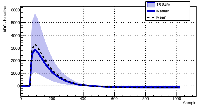
Run 039508 - Channel 2080 - 9682 waveforms
