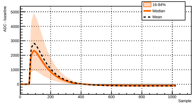
Run 039516 - Channel 2081 - 10764 waveforms
