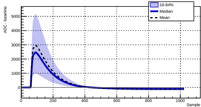
Run 039516 - Channel 2080 - 8775 waveforms
