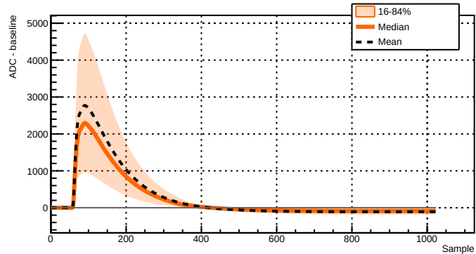
Run 039517 - Channel 2081 - 10810 waveforms
