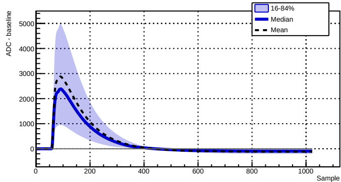
Run 039517 - Channel 2080 - 8769 waveforms
