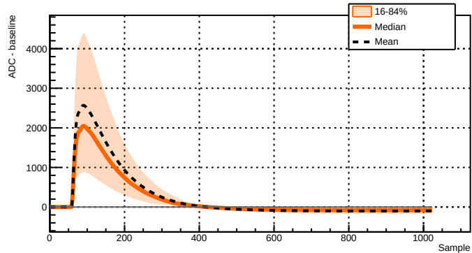
Run 039521 - Channel 2081 - 9962 waveforms
