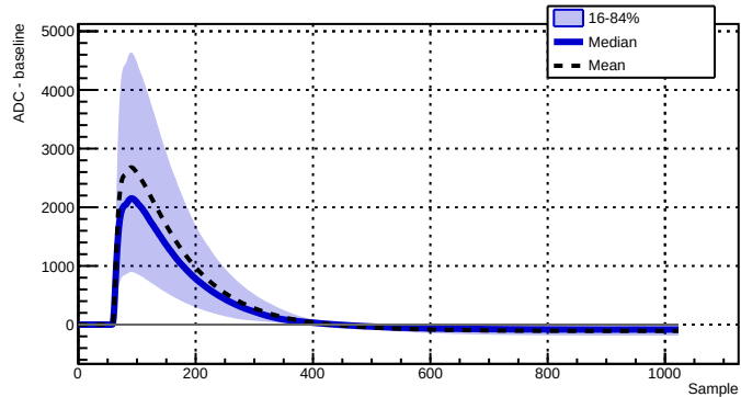
Run 039521 - Channel 2080 - 8013 waveforms
