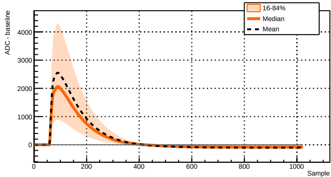
Run 039522 - Channel 2081 - 9776 waveforms
