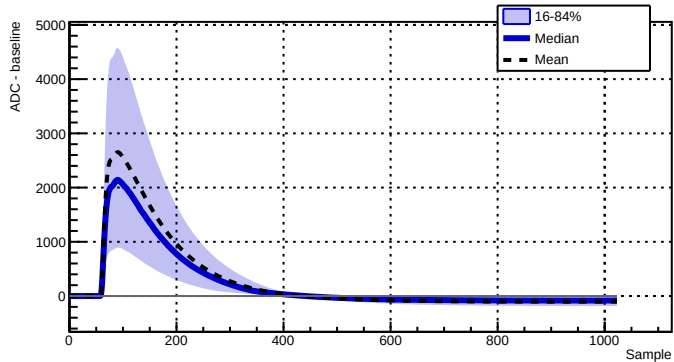
Run 039522 - Channel 2080 - 7866 waveforms
