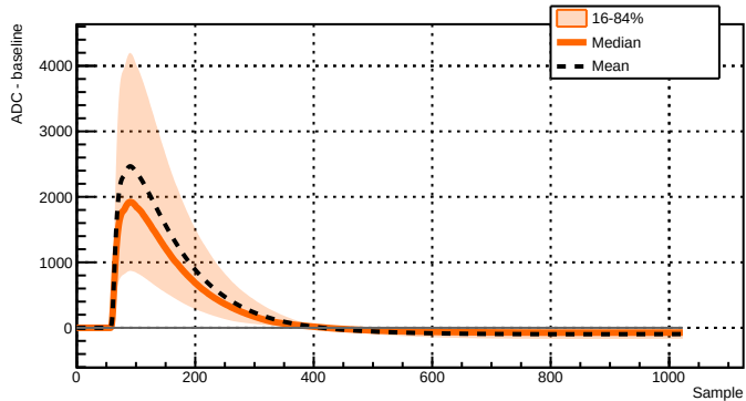
Run 039523 - Channel 2081 - 9424 waveforms
