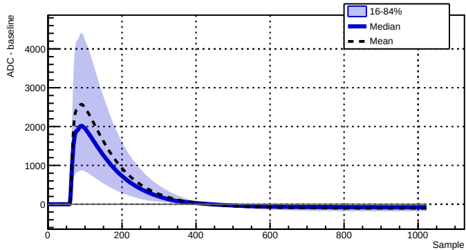
Run 039523 - Channel 2080 - 7640 waveforms
