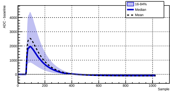
Run 039526 - Channel 2080 - 7304 waveforms
