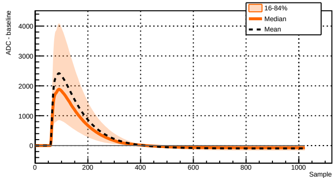
Run 039526 - Channel 2081 - 9111 waveforms
