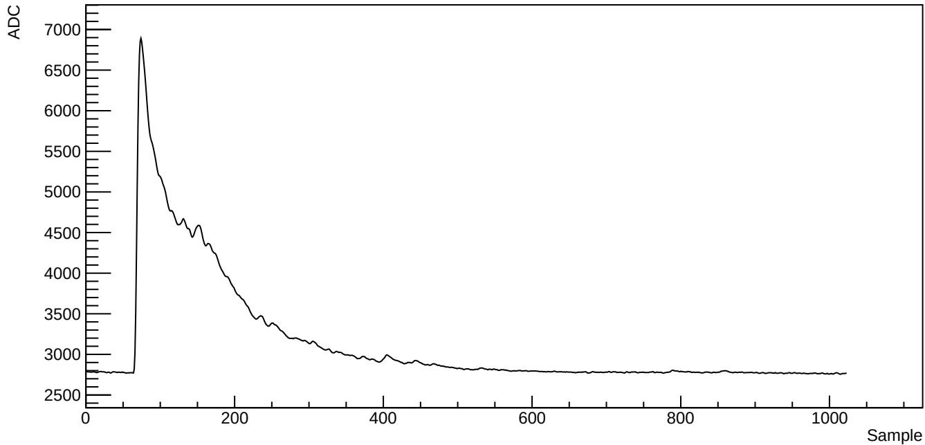
Run 39523, SubRun 1, Event 1, Channel 1010, Waveform index 737
