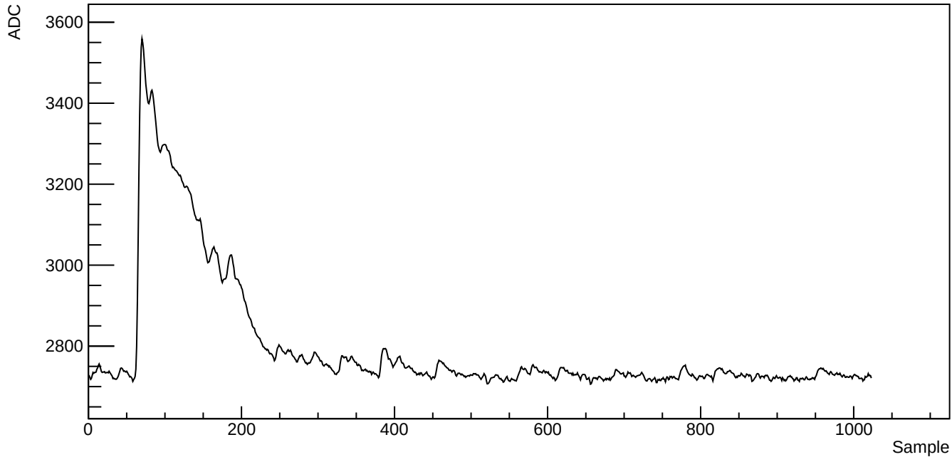
Run 39523, SubRun 1, Event 1, Channel 1010, Waveform index 763
