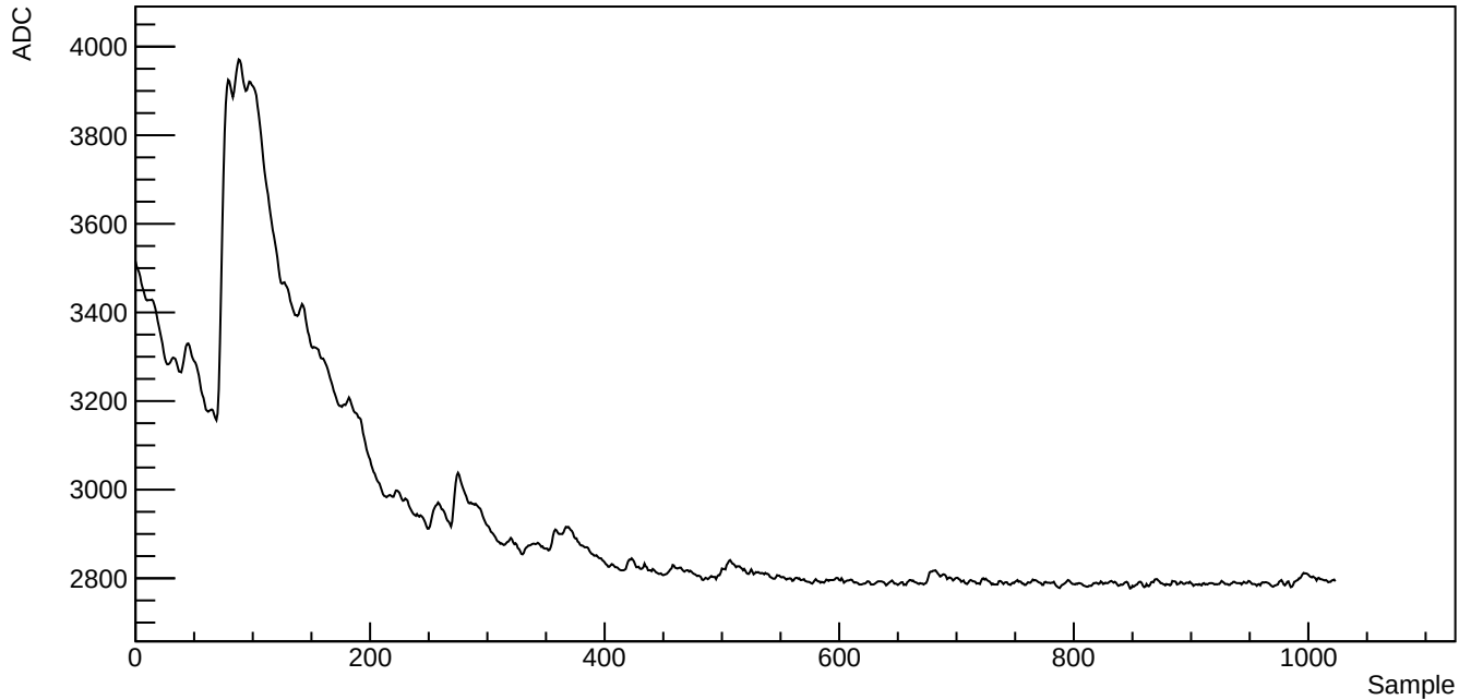
Run 39523, SubRun 1, Event 1, Channel 1010, Waveform index 729
