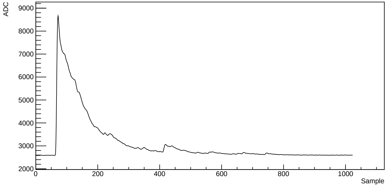
Run 39523, SubRun 1, Event 1, Channel 1010, Waveform index 748
