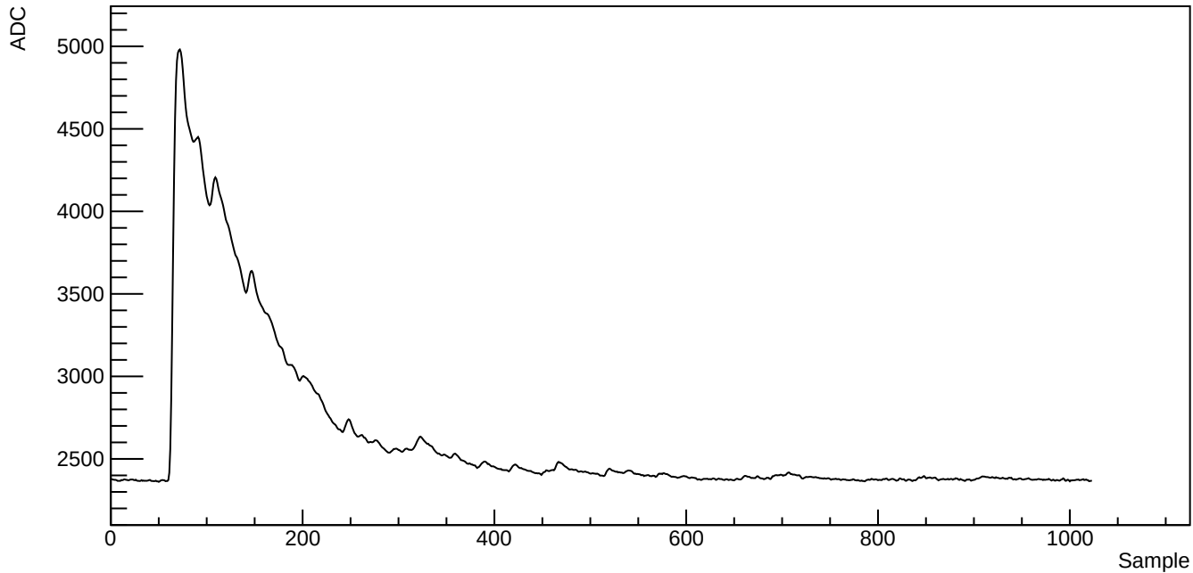
Run 39523, SubRun 1, Event 1, Channel 1010, Waveform index 746
