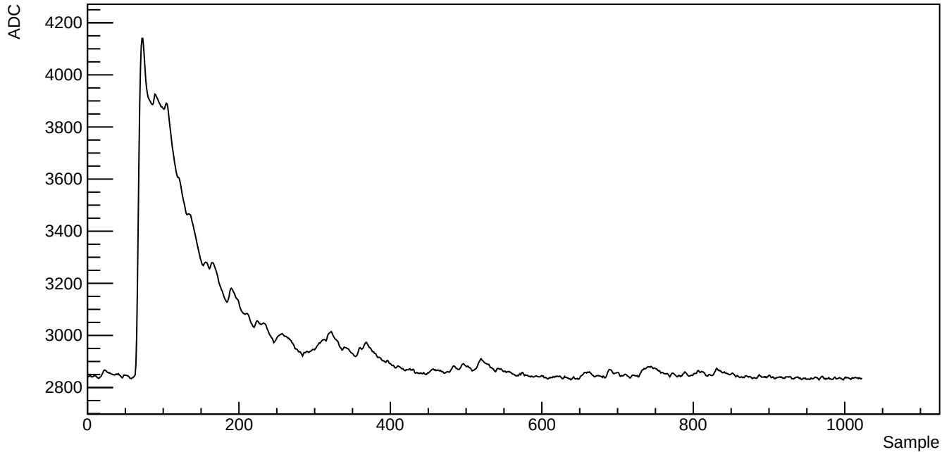
Run 39523, SubRun 1, Event 1, Channel 1010, Waveform index 732
