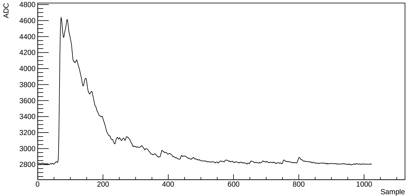
Run 39523, SubRun 1, Event 1, Channel 1010, Waveform index 767
