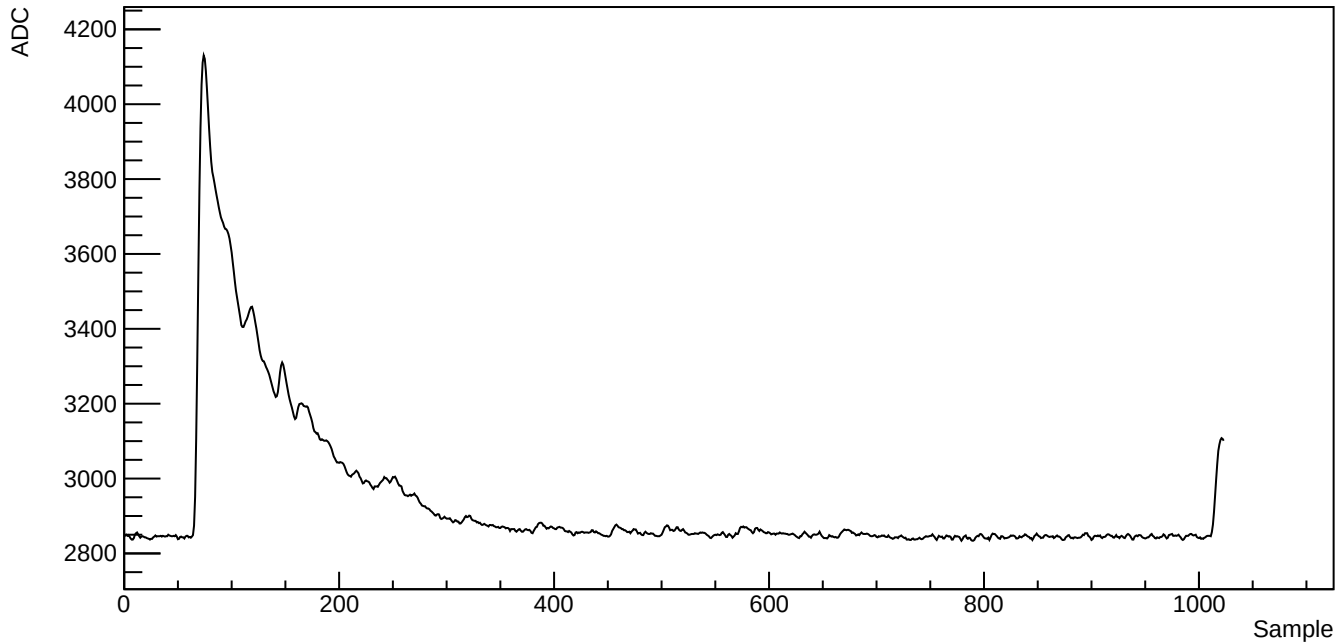
Run 39523, SubRun 1, Event 1, Channel 1010, Waveform index 736
