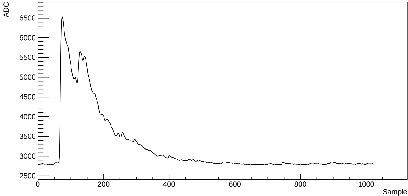
Run 39523, SubRun 1, Event 1, Channel 1010, Waveform index 727
