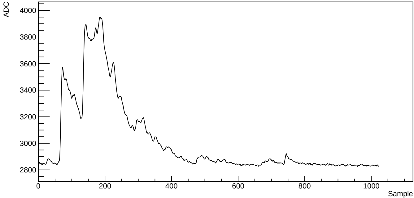
Run 39523, SubRun 1, Event 1, Channel 1010, Waveform index 731
