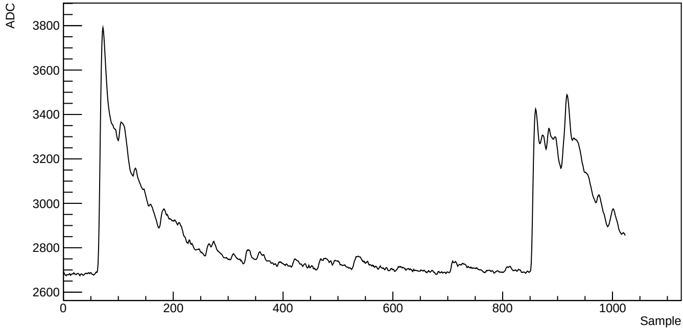
Run 39523, SubRun 1, Event 1, Channel 1010, Waveform index 756
