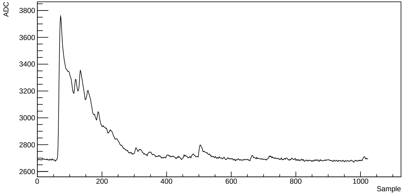
Run 39523, SubRun 1, Event 1, Channel 1010, Waveform index 753
