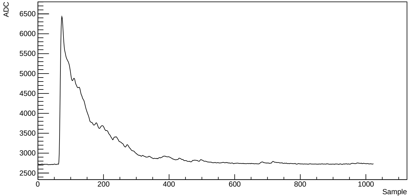
Run 39523, SubRun 1, Event 1, Channel 1010, Waveform index 764
