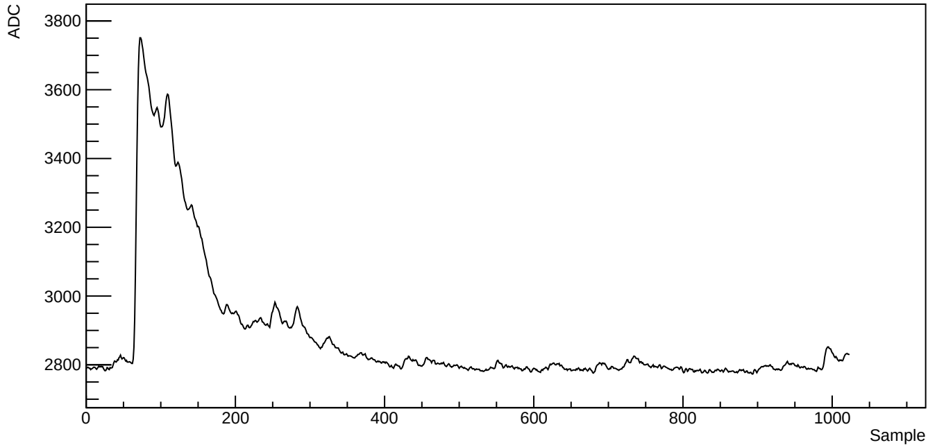
Run 39523, SubRun 1, Event 1, Channel 1010, Waveform index 724
