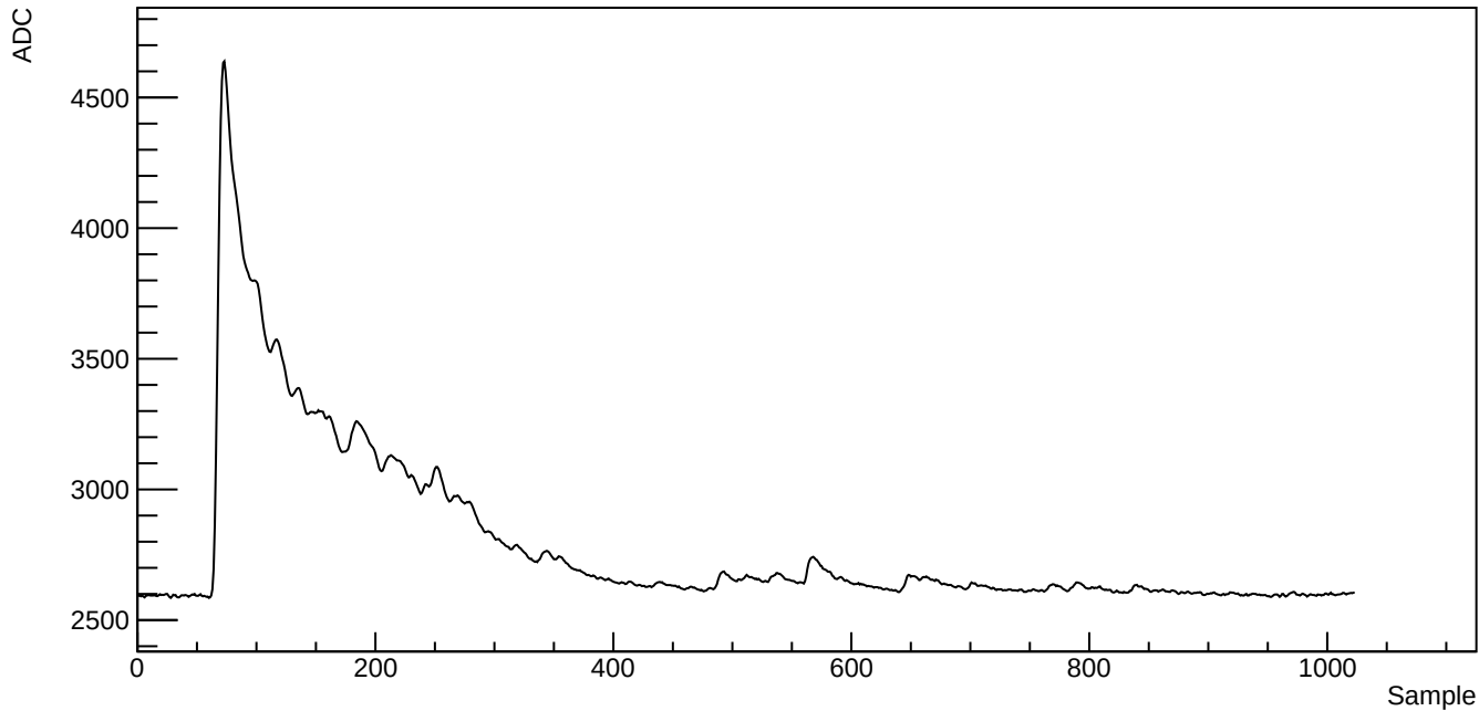
Run 39523, SubRun 1, Event 1, Channel 1010, Waveform index 760
