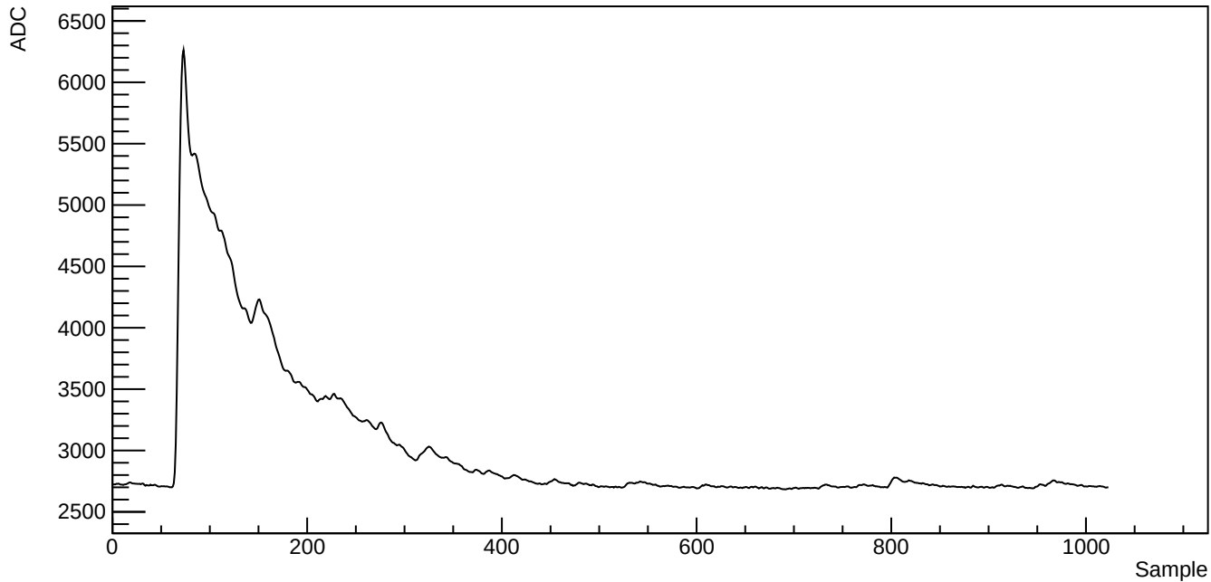
Run 39523, SubRun 1, Event 1, Channel 1010, Waveform index 757
