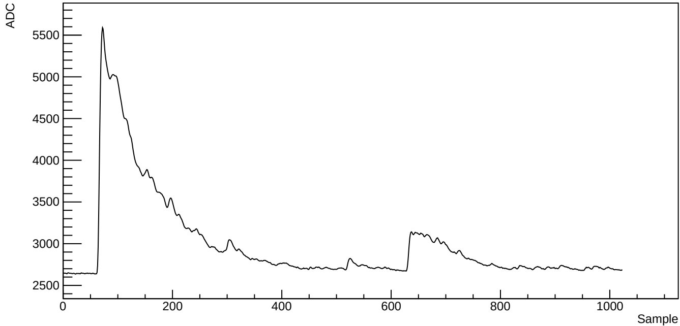
Run 39523, SubRun 1, Event 1, Channel 1010, Waveform index 749
