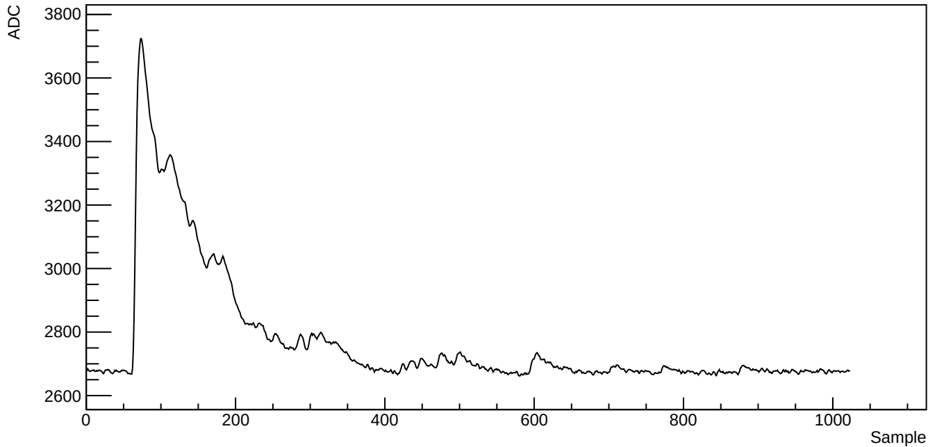
Run 39523, SubRun 1, Event 1, Channel 1010, Waveform index 739
