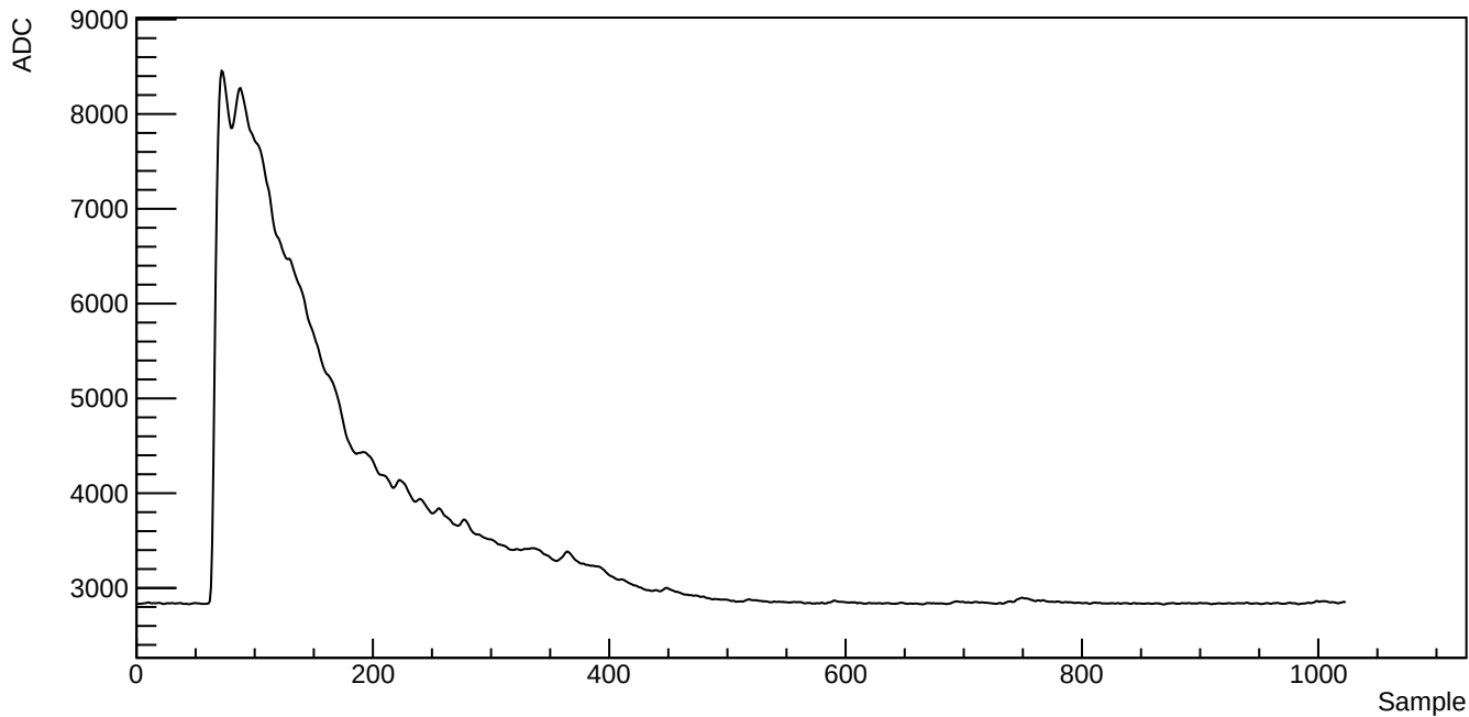
Run 39523, SubRun 1, Event 1, Channel 1010, Waveform index 734
