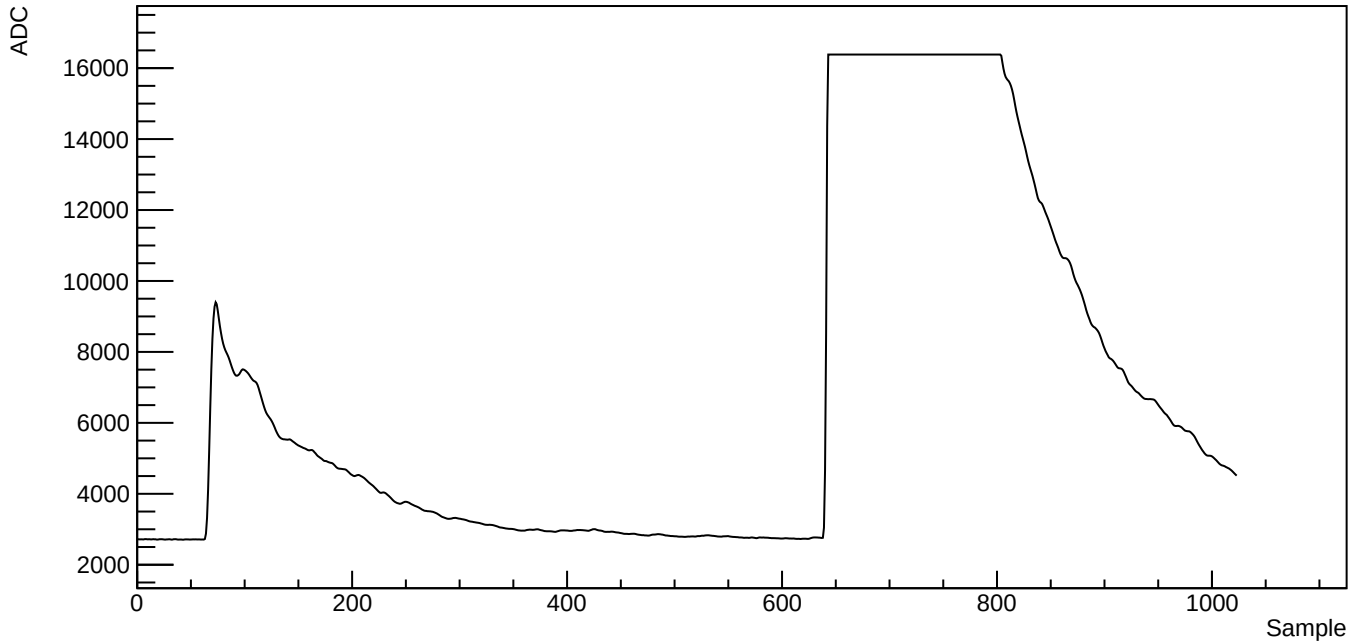
Run 39523, SubRun 1, Event 1, Channel 1010, Waveform index 759
