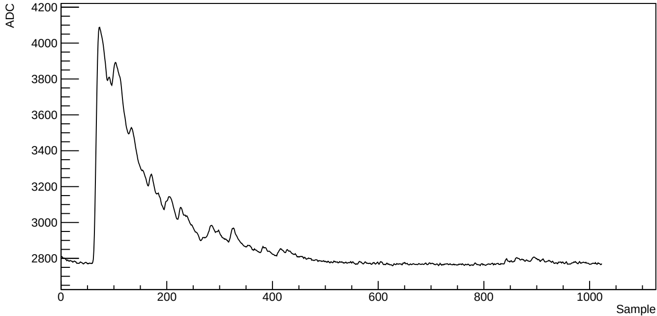
Run 39523, SubRun 1, Event 1, Channel 1010, Waveform index 765
