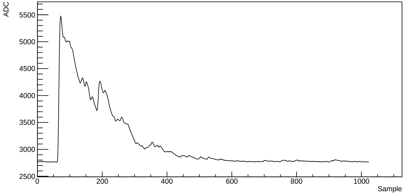
Run 39523, SubRun 1, Event 1, Channel 1010, Waveform index 769
