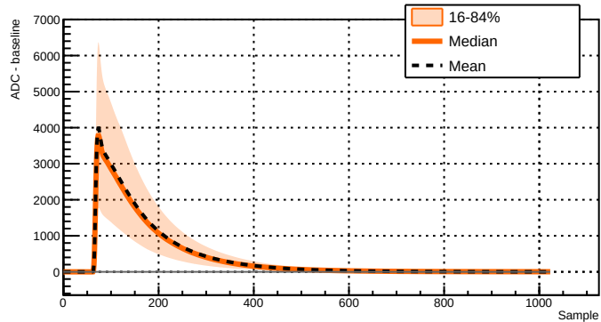
Run 039500 - Channel 1081 - 39046 waveforms
