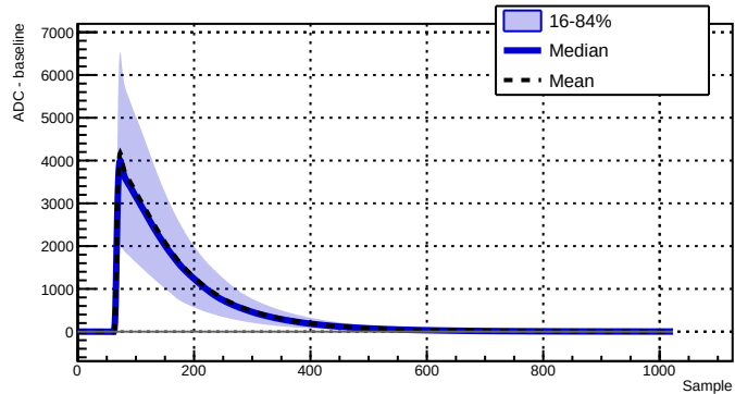
Run 039500 - Channel 1080 - 34184 waveforms
