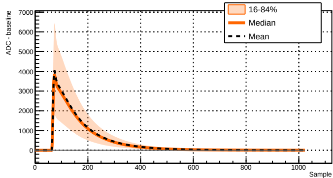
Run 039501 - Channel 1081 - 39197 waveforms
