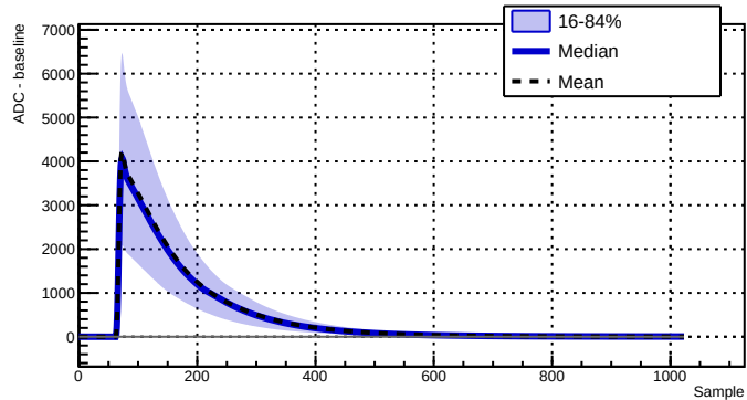
Run 039501 - Channel 1080 - 34183 waveforms
