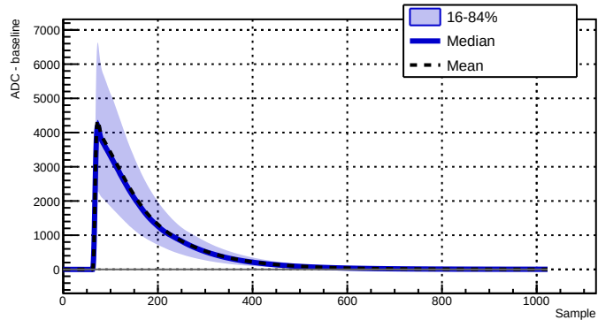
Run 039502 - Channel 1080 - 32456 waveforms
