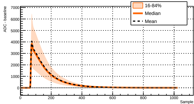
Run 039502 - Channel 1081 - 39284 waveforms
