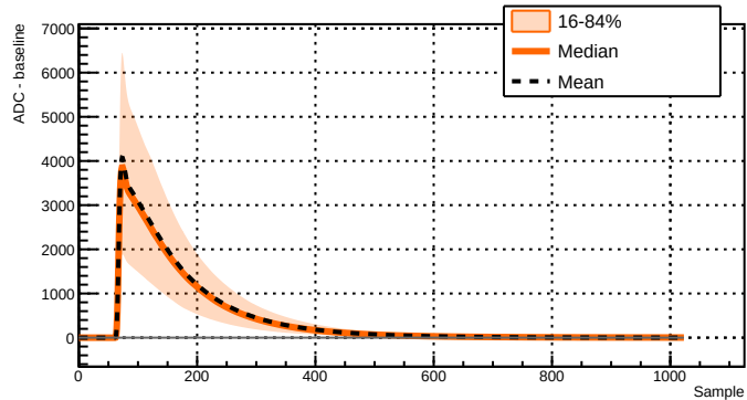
Run 039504 - Channel 1081 - 40196 waveforms
