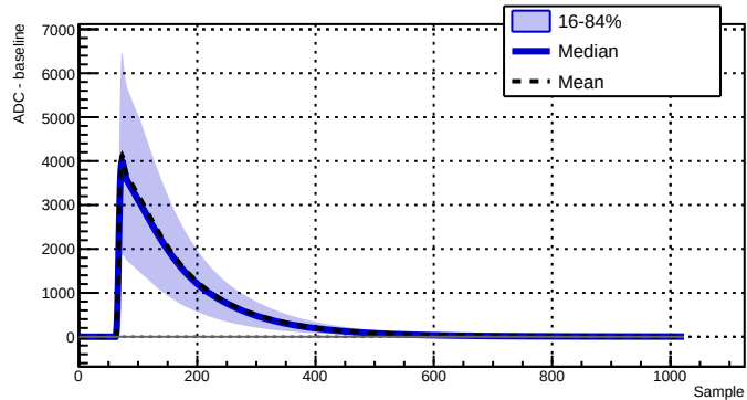
Run 039504 - Channel 1080 - 36756 waveforms
