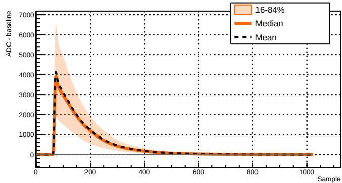
Run 039506 - Channel 1081 - 39948 waveforms
