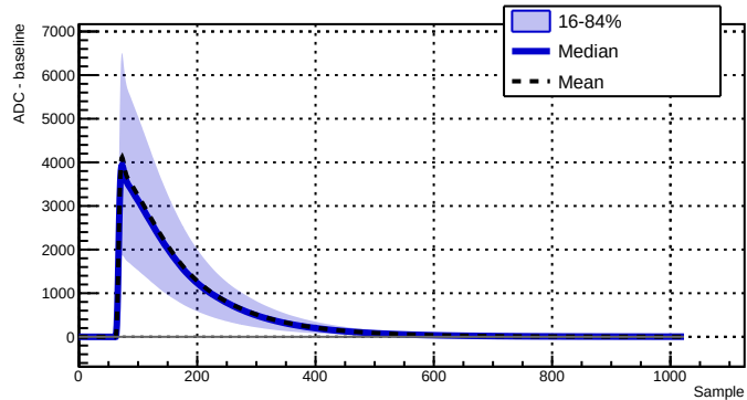
Run 039506 - Channel 1080 - 36623 waveforms
