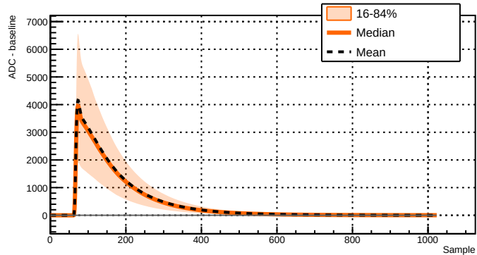
Run 039507 - Channel 1081 - 39289 waveforms
