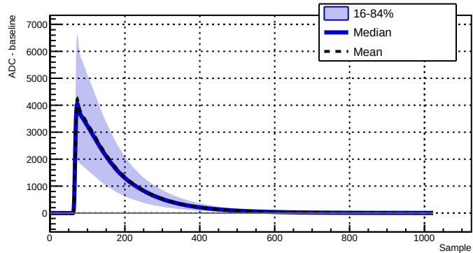
Run 039507 - Channel 1080 - 35662 waveforms
