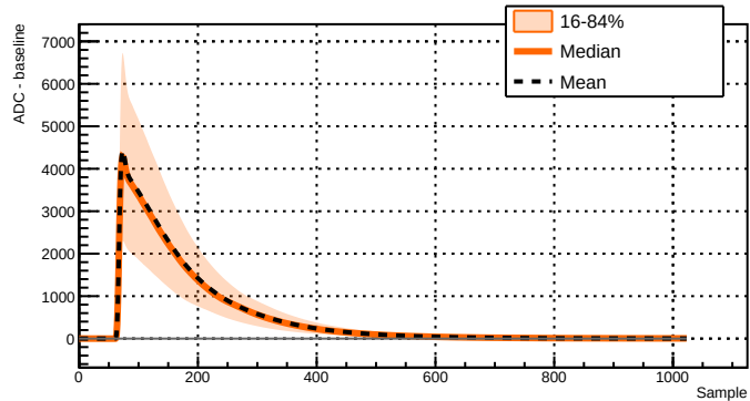
Run 039511 - Channel 1081 - 35417 waveforms
