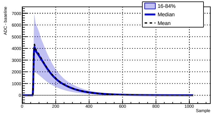
Run 039511 - Channel 1080 - 31426 waveforms
