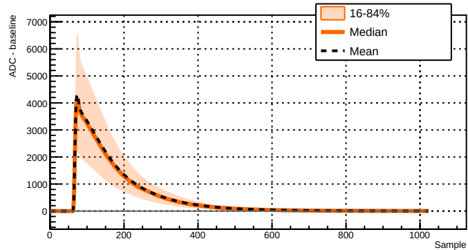
Run 039512 - Channel 1081 - 36470 waveforms
