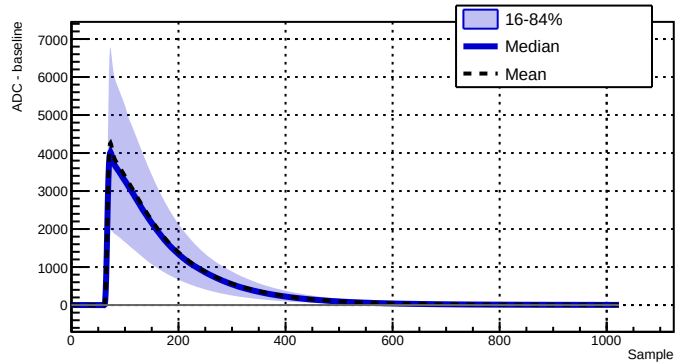
Run 039512 - Channel 1080 - 32909 waveforms
