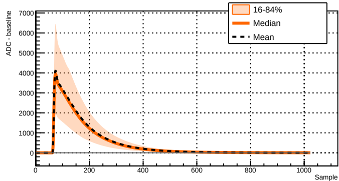
Run 039514 - Channel 1081 - 38537 waveforms
