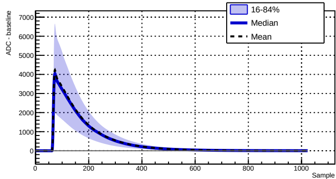
Run 039514 - Channel 1080 - 34363 waveforms
