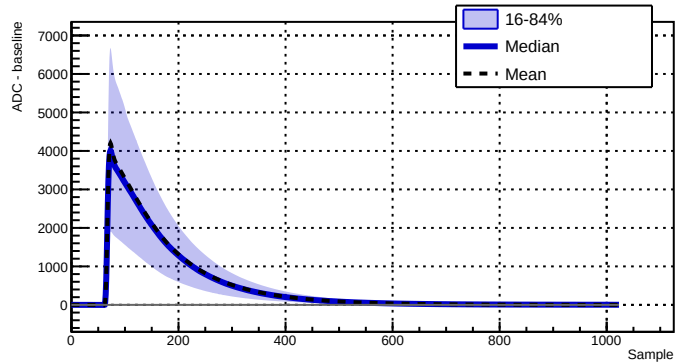
Run 039515 - Channel 1080 - 34038 waveforms
