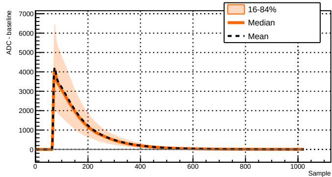
Run 039517 - Channel 1081 - 37755 waveforms
