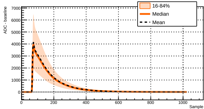
Run 039518 - Channel 1081 - 39450 waveforms
