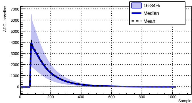
Run 039518 - Channel 1080 - 36850 waveforms
