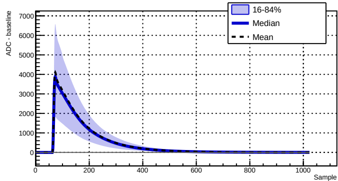
Run 039521 - Channel 1080 - 36258 waveforms
