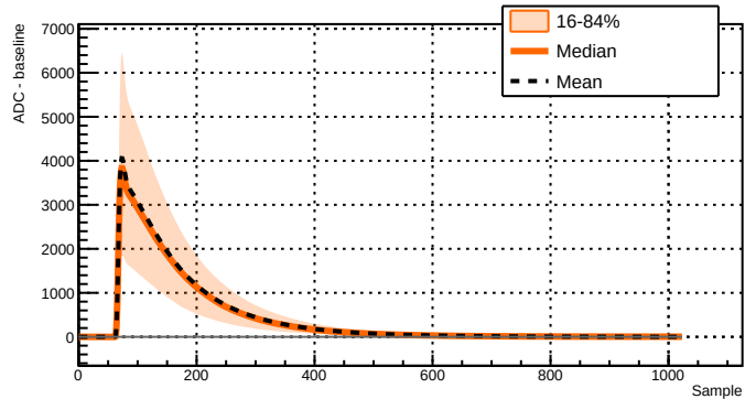
Run 039521 - Channel 1081 - 39374 waveforms
