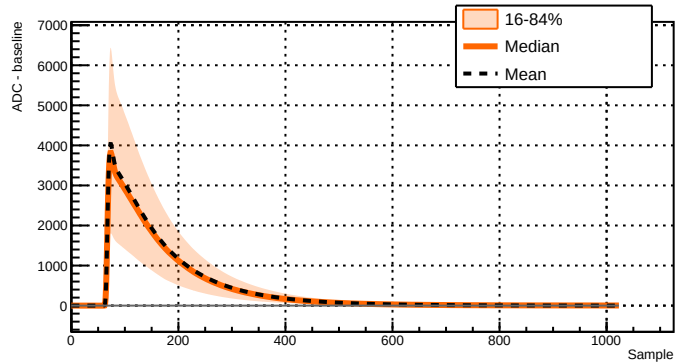
Run 039523 - Channel 1081 - 39947 waveforms
