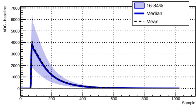
Run 039523 - Channel 1080 - 36845 waveforms
