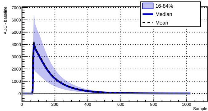
Run 039528 - Channel 1080 - 35013 waveforms
