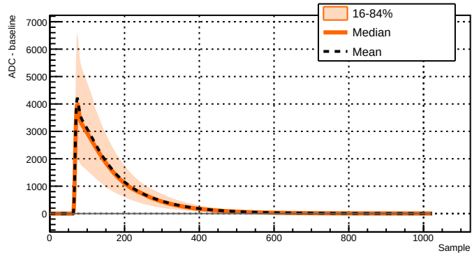
Run 039528 - Channel 1081 - 36268 waveforms
