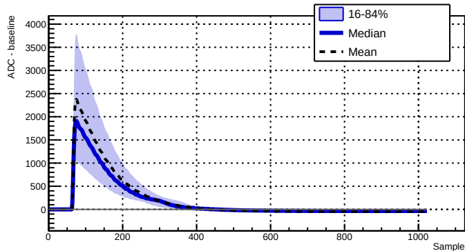
Run 039500 - Channel 2010 - 8023 waveforms
