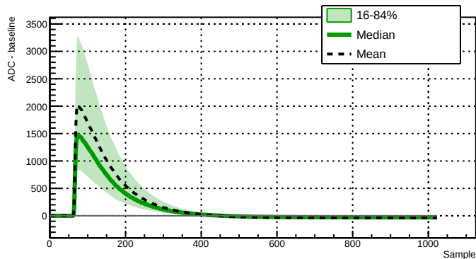
Run 039500 - Channel 2021 - 9454 waveforms
