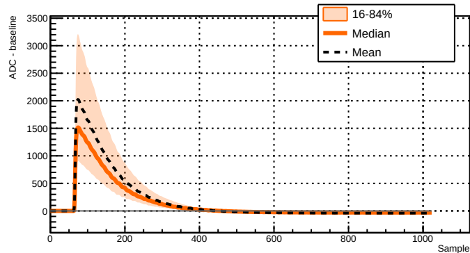
Run 039500 - Channel 2011 - 12684 waveforms
