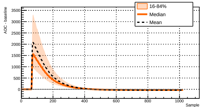
Run 039501 - Channel 2011 - 13741 waveforms
