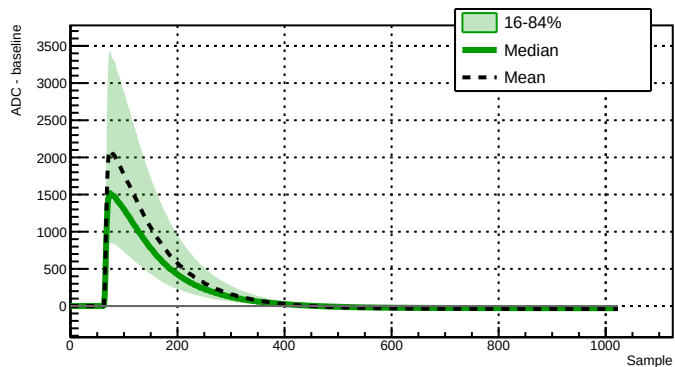
Run 039501 - Channel 2021 - 10215 waveforms
