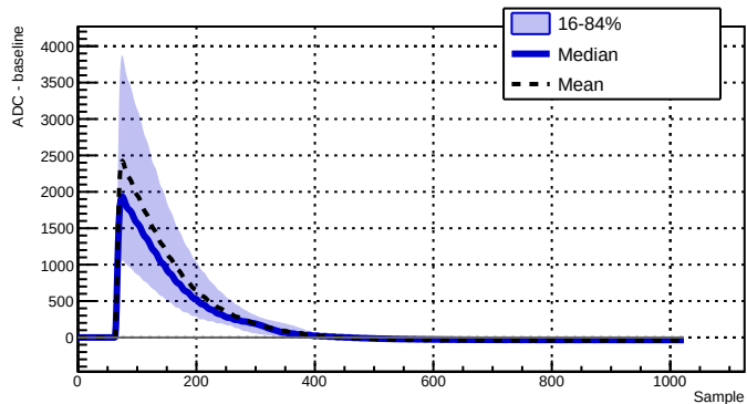
Run 039501 - Channel 2010 - 8977 waveforms
