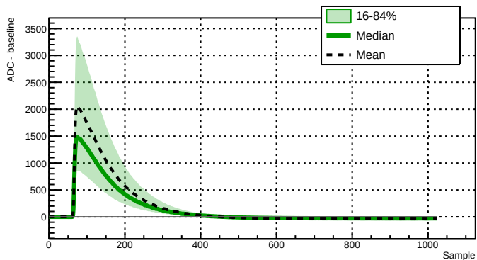
Run 039503 - Channel 2021 - 10419 waveforms
