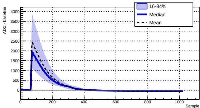
Run 039503 - Channel 2010 - 9263 waveforms
