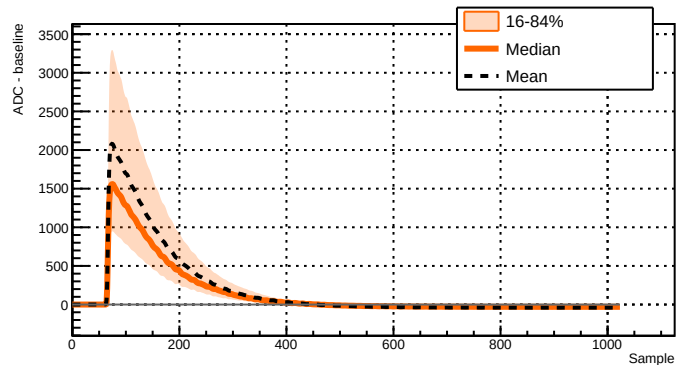
Run 039503 - Channel 2011 - 14084 waveforms
