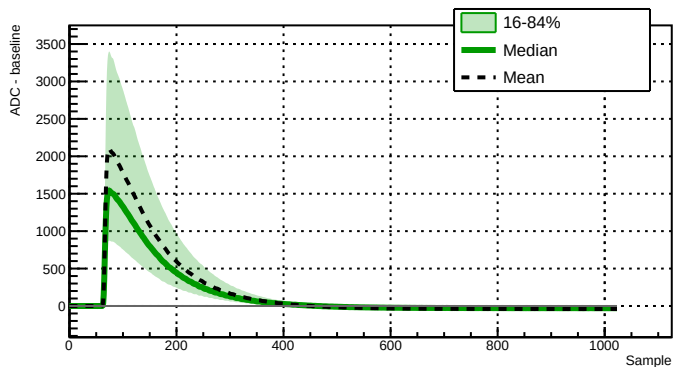
Run 039504 - Channel 2021 - 10278 waveforms
