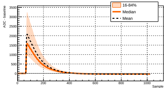
Run 039504 - Channel 2011 - 14055 waveforms
