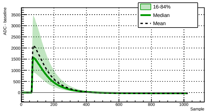
Run 039506 - Channel 2021 - 10238 waveforms
