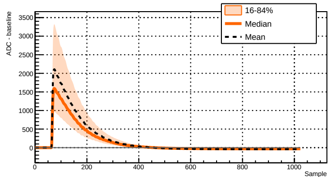
Run 039506 - Channel 2011 - 14437 waveforms
