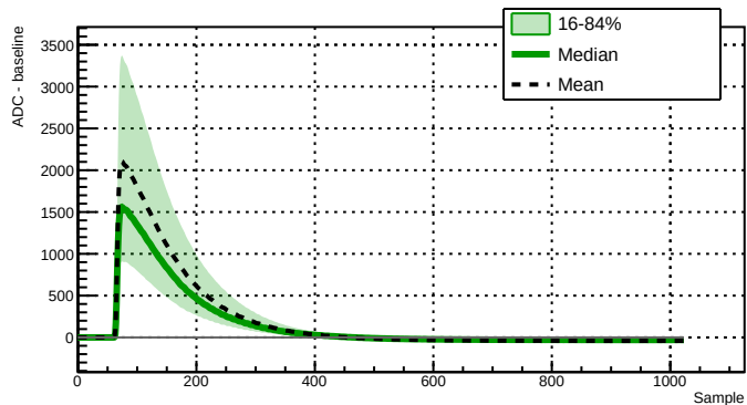
Run 039507 - Channel 2021 - 10353 waveforms
