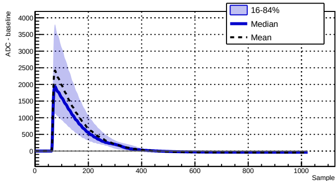
Run 039507 - Channel 2010 - 9439 waveforms
