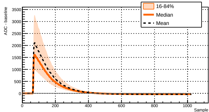
Run 039507 - Channel 2011 - 14303 waveforms
