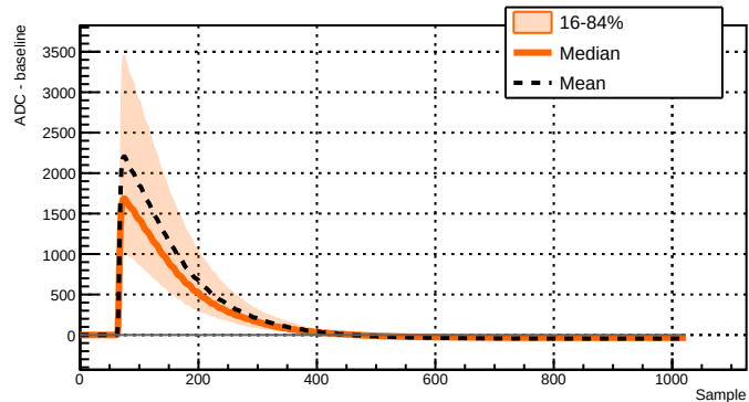
Run 039508 - Channel 2011 - 14257 waveforms
