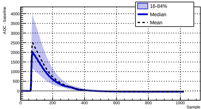
Run 039508 - Channel 2010 - 9637 waveforms
