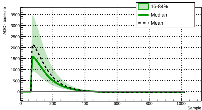
Run 039508 - Channel 2021 - 10769 waveforms
