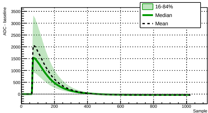
Run 039512 - Channel 2021 - 9999 waveforms
