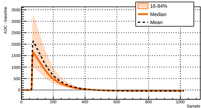
Run 039512 - Channel 2011 - 13206 waveforms
