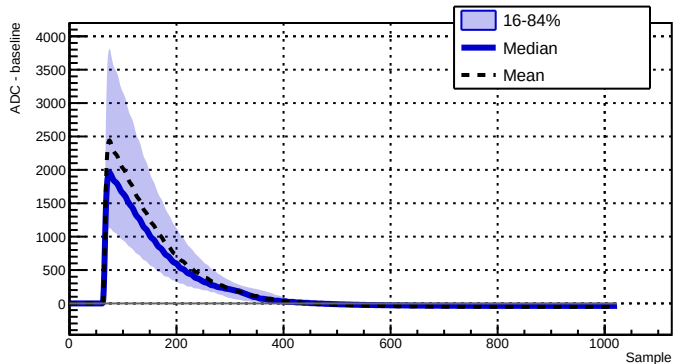
Run 039512 - Channel 2010 - 8564 waveforms
