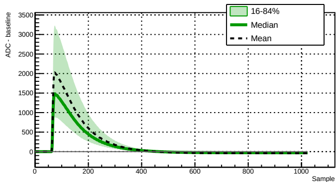
Run 039514 - Channel 2021 - 10049 waveforms
