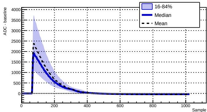
Run 039514 - Channel 2010 - 8374 waveforms
