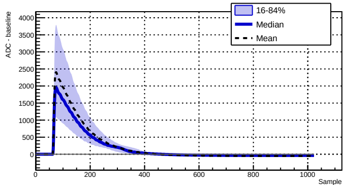
Run 039515 - Channel 2010 - 8092 waveforms
