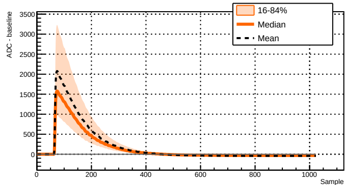
Run 039515 - Channel 2011 - 12991 waveforms
