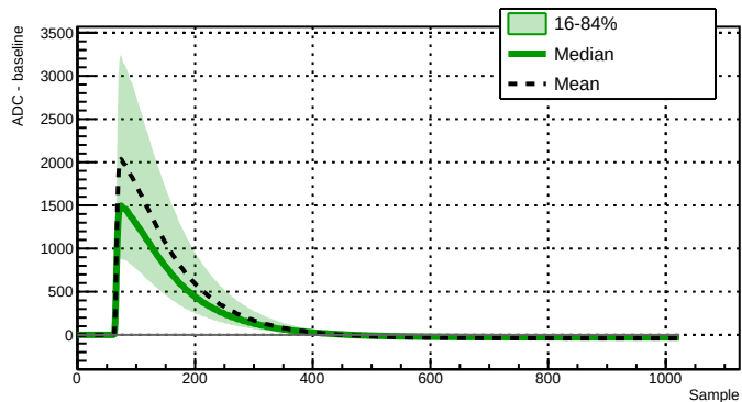
Run 039515 - Channel 2021 - 9805 waveforms
