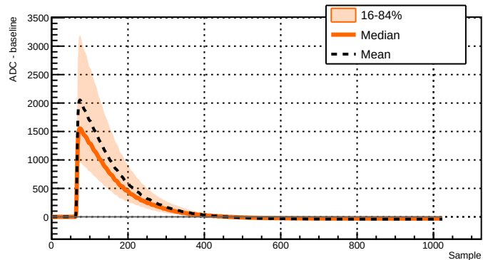
Run 039516 - Channel 2011 - 12850 waveforms
