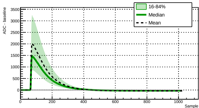
Run 039516 - Channel 2021 - 9759 waveforms
