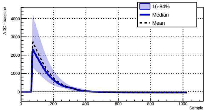
Run 039516 - Channel 2010 - 6117 waveforms
