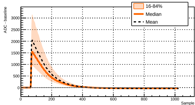
Run 039517 - Channel 2011 - 13501 waveforms
