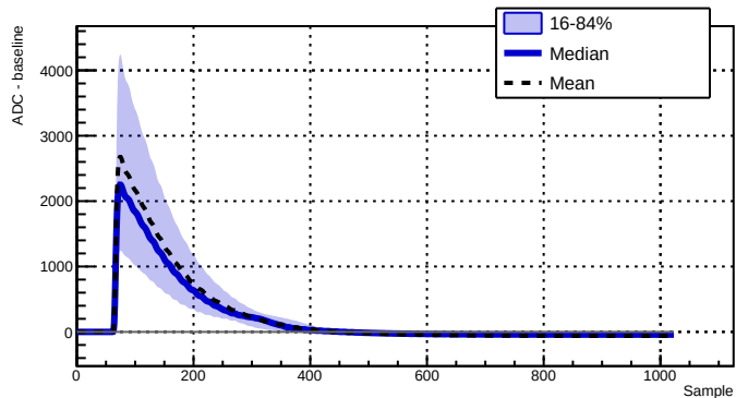
Run 039517 - Channel 2010 - 6532 waveforms
