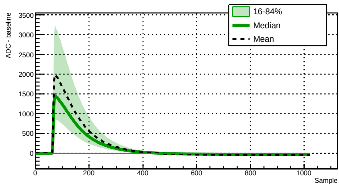
Run 039517 - Channel 2021 - 10404 waveforms
