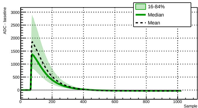
Run 039518 - Channel 2021 - 10013 waveforms
