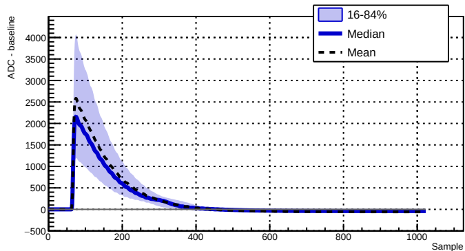
Run 039518 - Channel 2010 - 6270 waveforms
