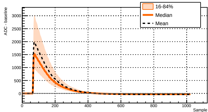
Run 039518 - Channel 2011 - 12961 waveforms
