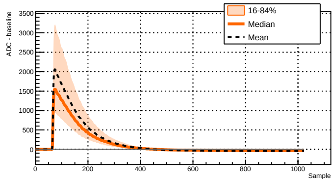
Run 039522 - Channel 2011 - 13915 waveforms
