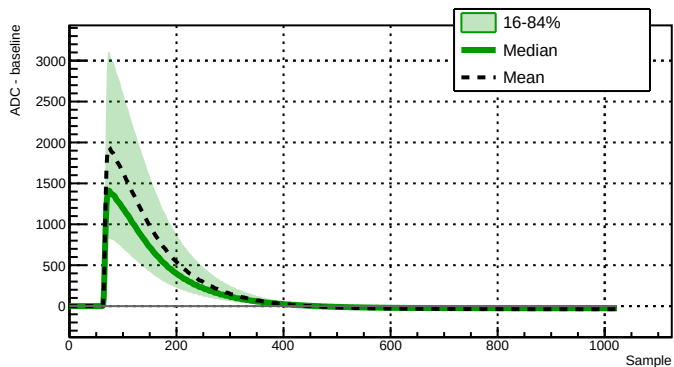
Run 039522 - Channel 2021 - 10762 waveforms
