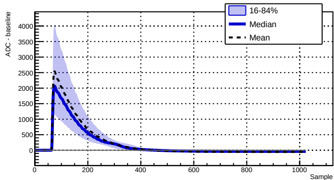
Run 039523 - Channel 2010 - 7422 waveforms
