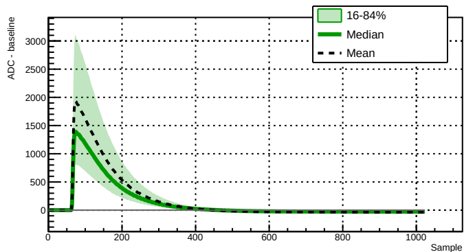
Run 039523 - Channel 2021 - 10817 waveforms
