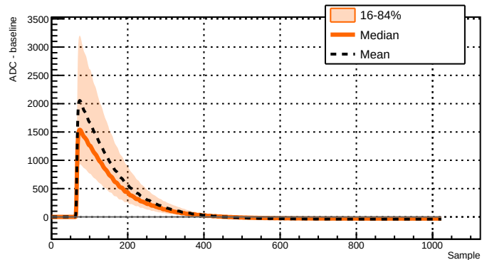
Run 039523 - Channel 2011 - 13818 waveforms
