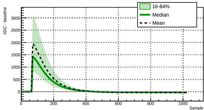
Run 039525 - Channel 2021 - 10602 waveforms
