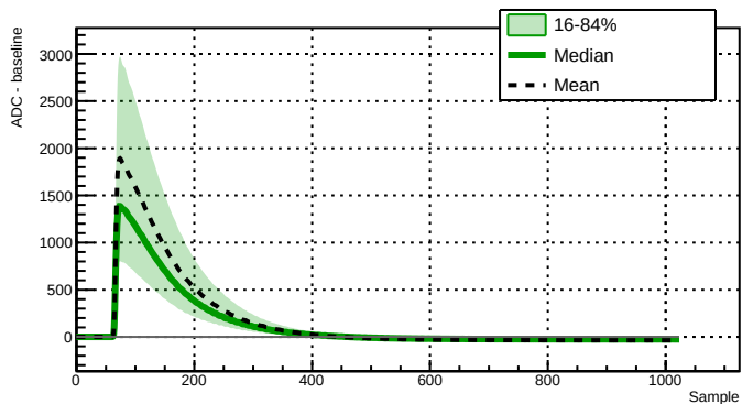
Run 039527 - Channel 2021 - 10352 waveforms
