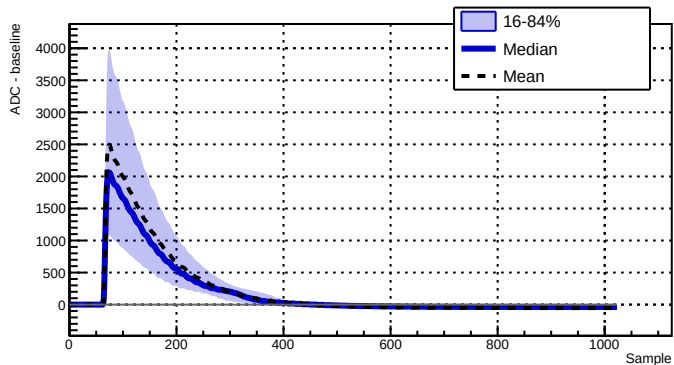
Run 039527 - Channel 2010 - 6984 waveforms
