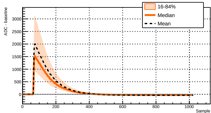
Run 039527 - Channel 2011 - 13309 waveforms
