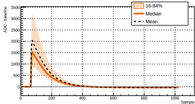
Run 039528 - Channel 2011 - 13213 waveforms
