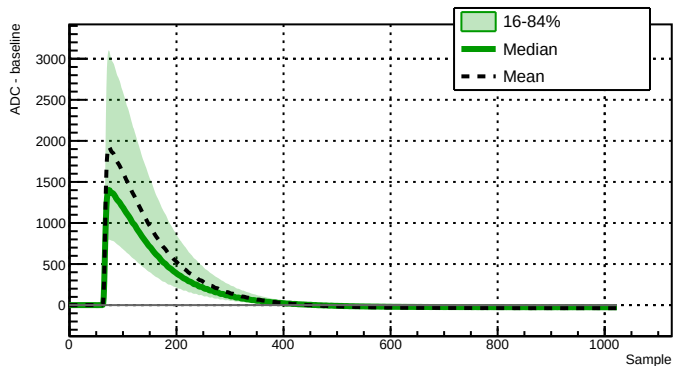
Run 039528 - Channel 2021 - 10290 waveforms
