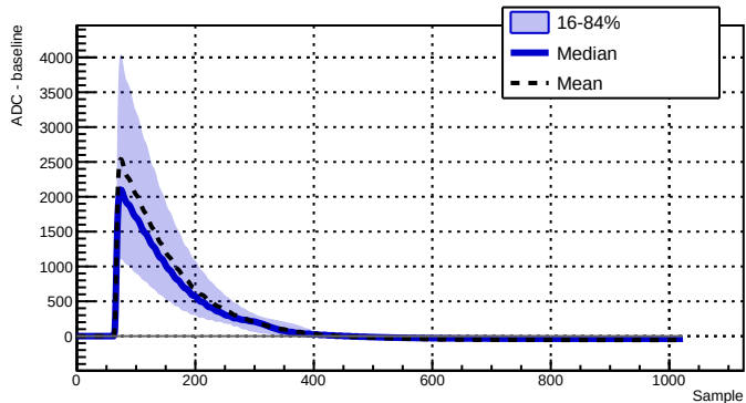
Run 039528 - Channel 2010 - 7025 waveforms
