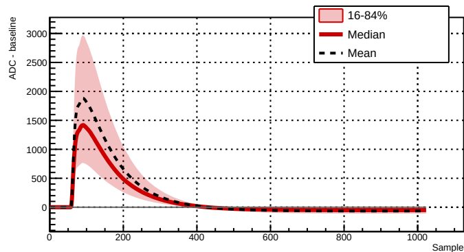
Run 039500 - Channel 2081 - 24320 waveforms
