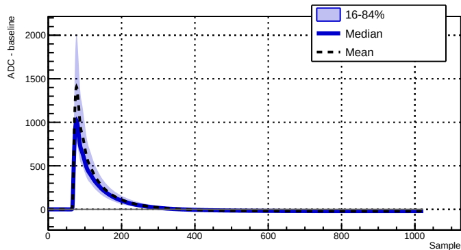
Run 039500 - Channel 2070 - 8915 waveforms
