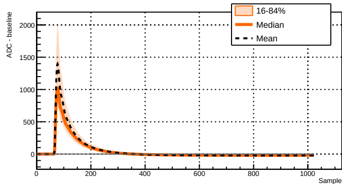
Run 039500 - Channel 2071 - 8558 waveforms
