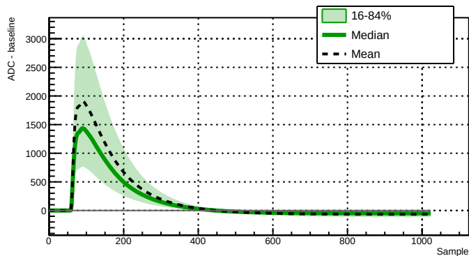
Run 039500 - Channel 2080 - 24166 waveforms
